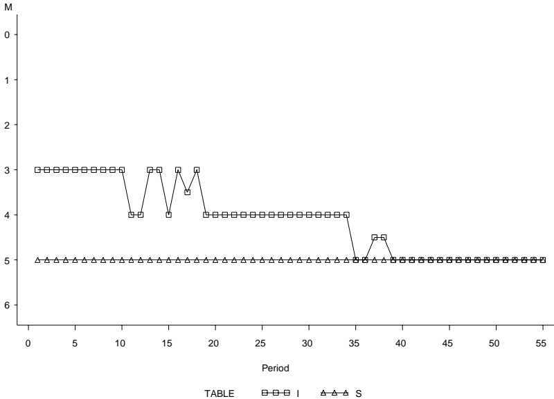
Figure 3: Median actions for I(0,1) "□" and S(0,1) "Δ" sessions.
