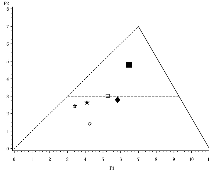
Figure 6: The average payoff in the last five periods of \Gamma(0,1) "☆" or "★" and the initial, "□" or "■", and terminal periods, "◇" or "◆", of the last \Gamma(5/6,2) match. Solid symbols denote S treatments and hollow symbols denote I treatments
