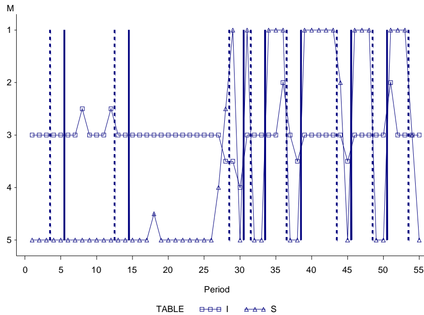
Figure 5: Median action in I(5/6,2) " \square " and S(5/6,2) " \triangle ". Dashed vertical line denotes transition to terminal phase and solid vertical line denotes rematching.
