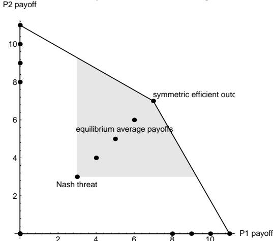
Figure 1: Convex hull of feasible payoffs in games I and S .
