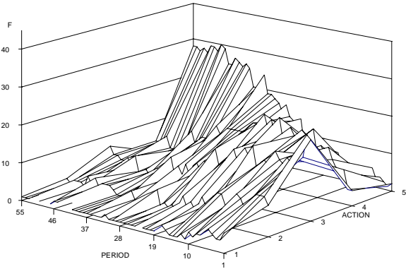
Figure 4a: Frequency distribution of actions observed in I(0,1) by period.
