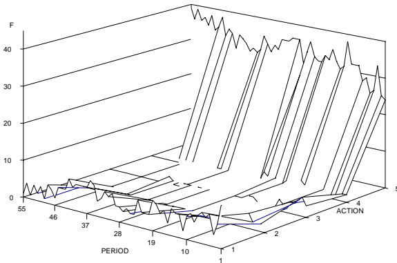
Figure 4b: Frequency distribution of actions observed in S(0,1) by period.
