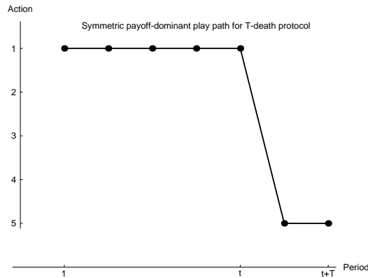
Figure 2: Observable actions of symmetric payoff-dominant equilibrium play path.
